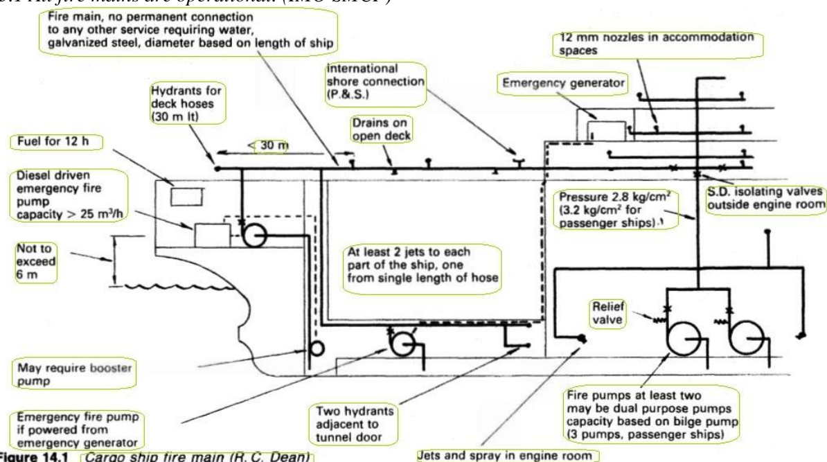
Figure 14.1 Cargo ship fire main (R. C. Dean)
