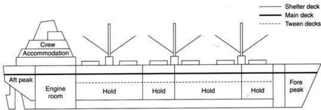
Fig. 16.16 The shelter deck vessel
