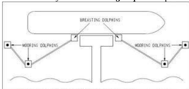
Breasting dolphin and mooring dolphin http://www.engineeringcivil.com
