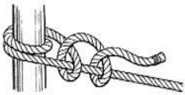
Round Turn With Two Half Hitches
