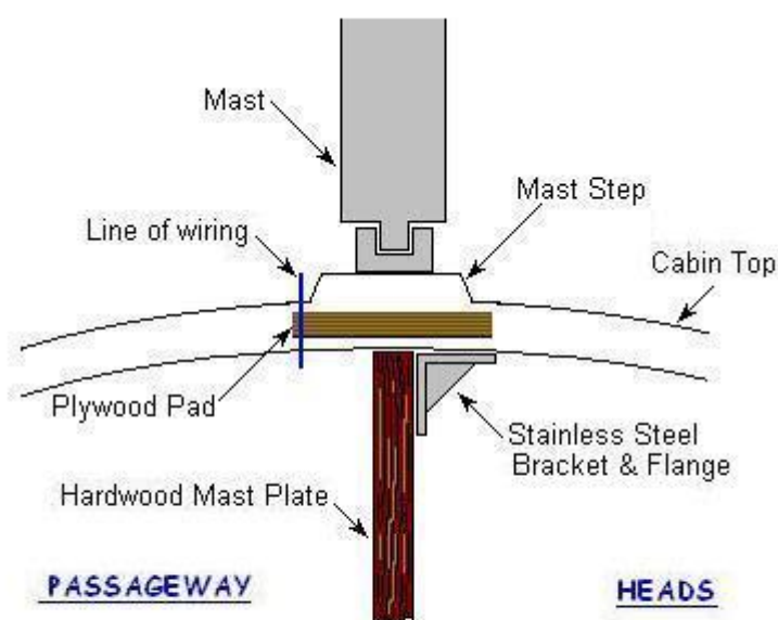
Sketch of Mast Support ( Not to Scale )
