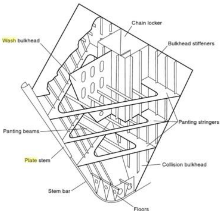
FIGURE 20.2 Fore end structure
