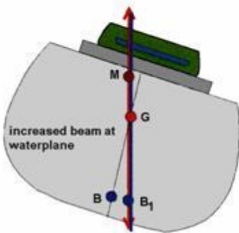
3. Stable at the angle of loll
