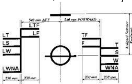
Figure 4: Timber Load Line Marking Lines to be used with this mark.
