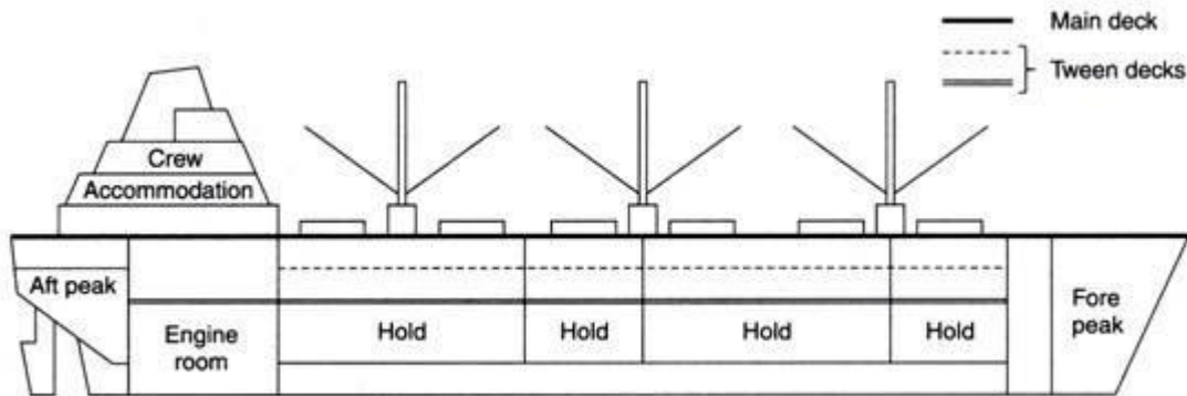
Fig. 16.15 The tween deck vessel (with cargo gear)
