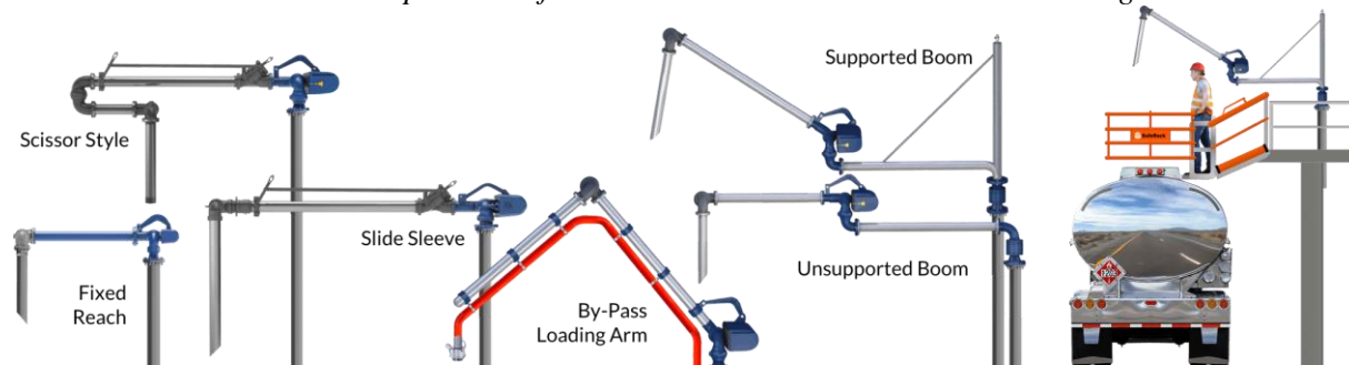
Top Loading Arms - Common Types
