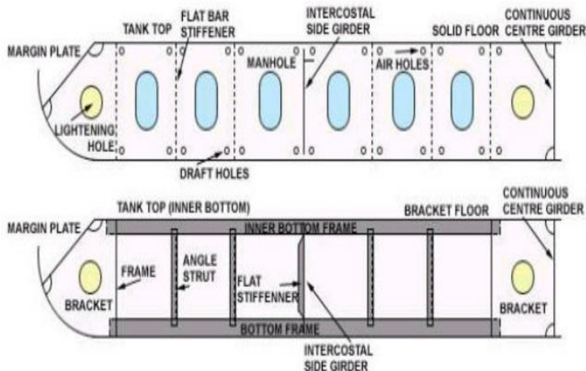
FIGURE 10 Transversely framed double bottom construction
