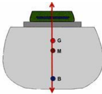
1. Unstable equilibrium
