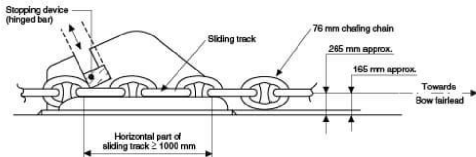
Bar hinged type chain stopper
